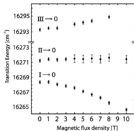
Figure 7. Magnetic field induced shifts of the T_1 substates I, II, and III of \text{Ir}(\text{btp})_2(\text{acac}) in \text{CH}_2\text{Cl}_2 (site H). The data are extracted from emission spectra recorded at various temperatures in the range from 2.8 to 14 K. The emission lines corresponding to transition I_B \rightarrow 0 were determined at T = 2.8 \text{ K} , while the emission from the substates II_B and III_B was measured at 8 and 14 K, respectively. The higher temperature was chosen to provide sufficient population of these states. For recording emission from substates I and II, substate III was excited, while emission from substate III was measured under excitation into a vibrational satellite of substate III ( \bar{\nu}_{\text{exc}} = 16742 \text{ cm}^{-1} at B = 0 \text{ T} ). Selective excitation was always tuned with increasing magnetic field strength to match the excitation energy of the Zeeman shifted state III.
