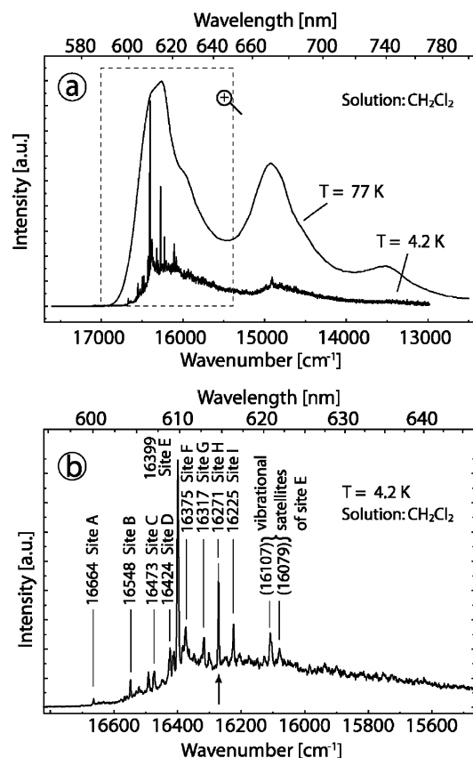
Figure 2. (a) Comparison of the emission spectra of Ir(btp) 2 (acac) in CH 2 Cl 2 (10 -5 mol/L) recorded at 77 and 4.2 K, respectively, excited at \lambda_{\text{exc}} = 363.8 nm. At 77 K, the spectrum is still unresolved due to inhomogeneous broadening and homogeneous broadening by electron–phonon coupling. The 4.2 K spectrum shows a site structure consisting mainly of highly resolved electronic 0–0 lines and an intense inhomogeneous background. (b) Magnified region of the 4.2 K emission framed in part a. All lines labeled with capital letters represent electronic origins (T 1 substate II → ground state S 0 ) of different sites. In particular, site H at 16271 cm -1 (arrow in part b) will be subject to detailed investigations in the following sections.
