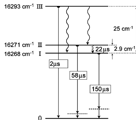
Figure 5. Energy level diagram and photophysical data for the lowest triplet state T_1 of Ir(btp) 2 (acac). The state is classified as ^3\text{LC} state which is strongly MLCT perturbed. The values given apply to the specific site under investigation (site H in Figure 2b). Other sites display different values (compare Table 1). After excitation of triplet substate III, the relaxation to the lower lying substates (spin–lattice relaxation, SLR) is fast even at T = 1.2 \text{ K} . However, the relaxation time between the substates II and I is extremely long and amounts to \tau_{\text{SLR}} = 22 \mu\text{s} at T = 1.5 \text{ K} . This value and the individual decay times are determined in ref 38 and are given here for completeness. The dashed lines represent vibrational levels, which are usually also involved in the emission processes.
