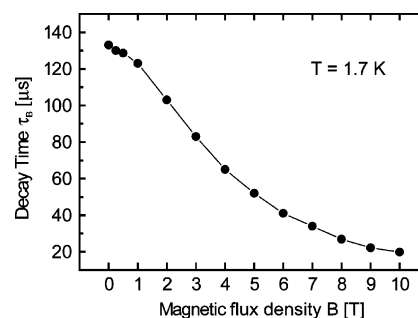
Figure 8. Emission decay time of \text{Ir}(\text{btp})_2(\text{acac}) in \text{CH}_2\text{Cl}_2 (site H). The decay time is measured for different magnetic flux densities B at T = 1.7 \text{ K} and under selective excitation of T_1 substate III. The decay behavior is monoexponential in the whole range 0 \leq B \leq 10 \text{ T} .
